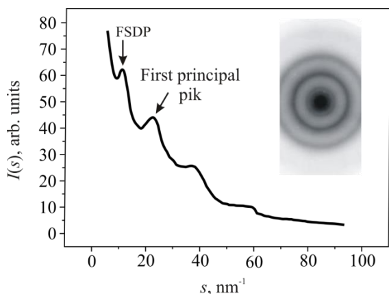
Fig 1. Typical diffractogram and electronogram (inset) of the amorphous substances (in this case – the amorphous As_{40}Se_{60} film)
